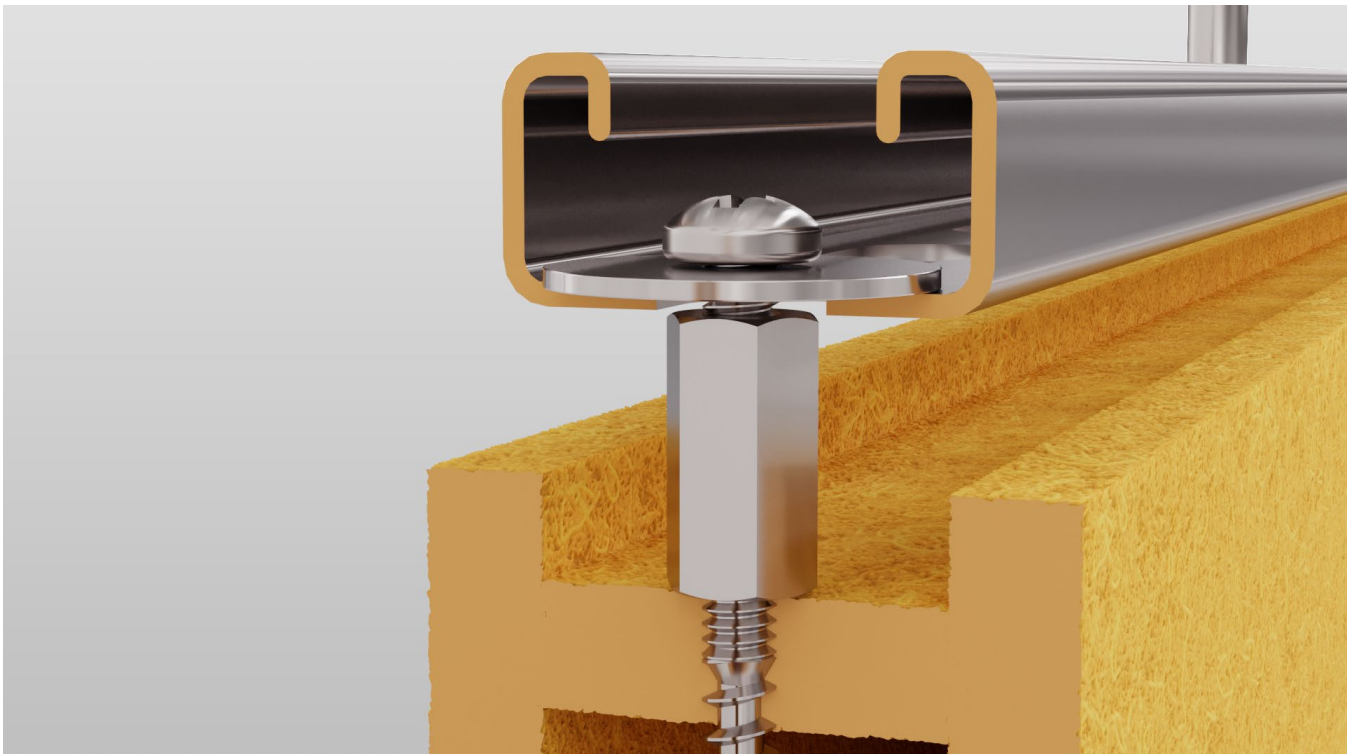
Direct mount to Unistrut with Bolt (male), Coupler, Washer, and Screw
