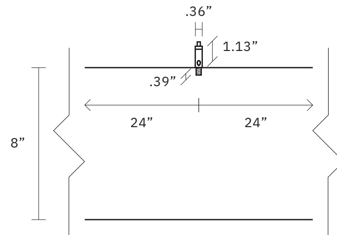
Hardware Cross Section Detail View
